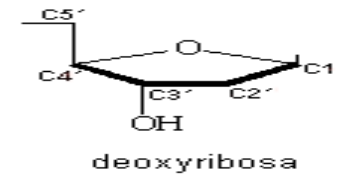
deoxyribosa
