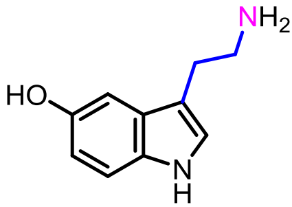
Serotonin
