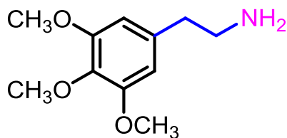
Mescaline hallucinations
