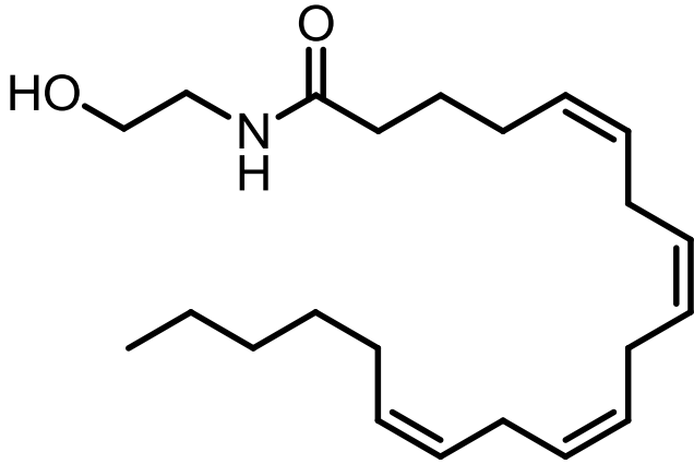
Anandamide
