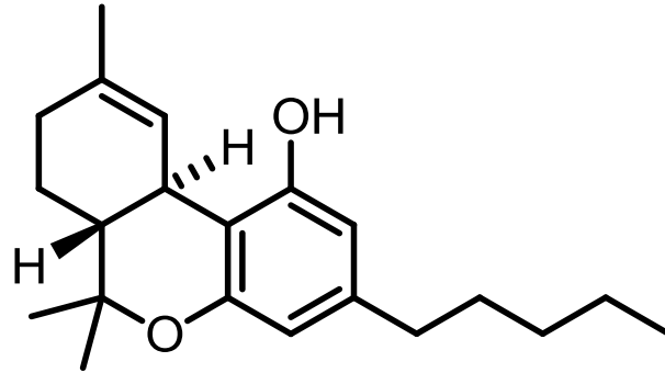
Tetrahydrocannabinol (THC)
